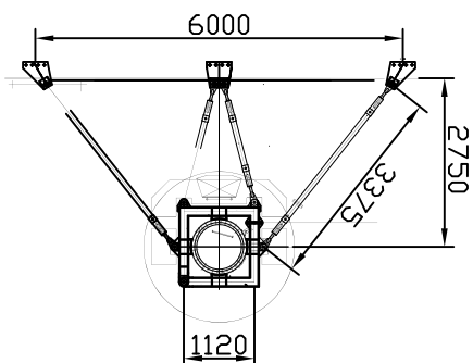
Typical wall tie
